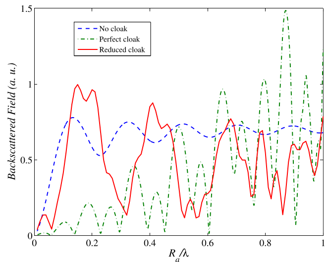
FIG. 2. Frequency dependence of the backscattered field produced by a rigid cylinder with radius R_a (dashed line) and its comparison with the fields produced by the cylinder surrounded with a perfect cloak made of a layered shell with 20 layers [6] (dotted line) and by the 20 layers thick reduced cloak proposed here (continuous line).
