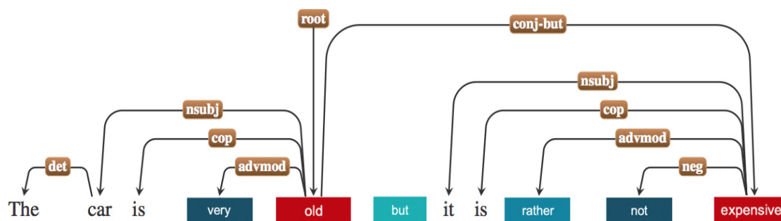
(a) Dependency tree of a sentence.
