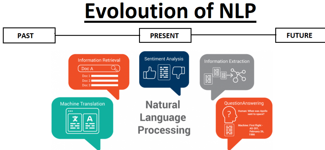
Figure 6.1: NLP applications [27]
