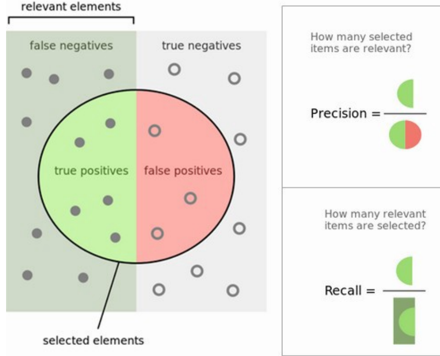
Figure 5.1: Precision and recall measures [2]
