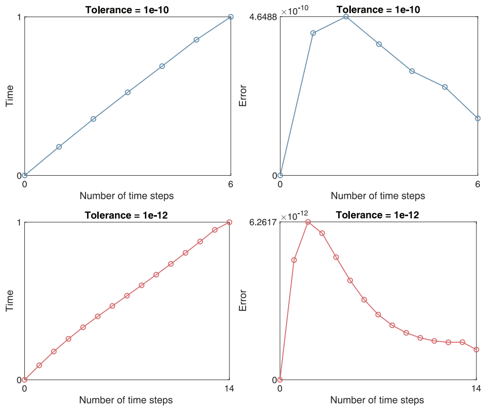
FIGURE 6. Corresponding results for a sixth-order symmetric-conjugate splitting method and lower tolerances 10^{-10} and 10^{-12} , respectively.
