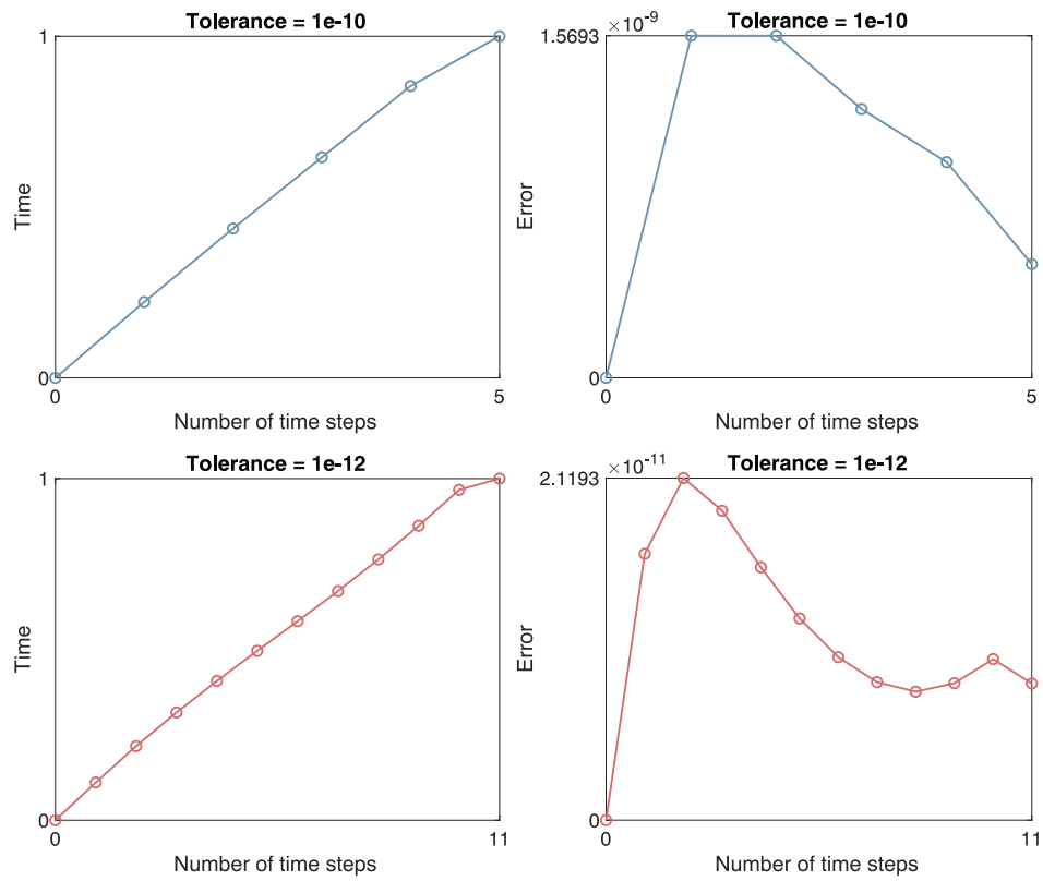
FIGURE 8. Corresponding results for the sixth-order symmetric-conjugate splitting method with respect to the maximum norm.
