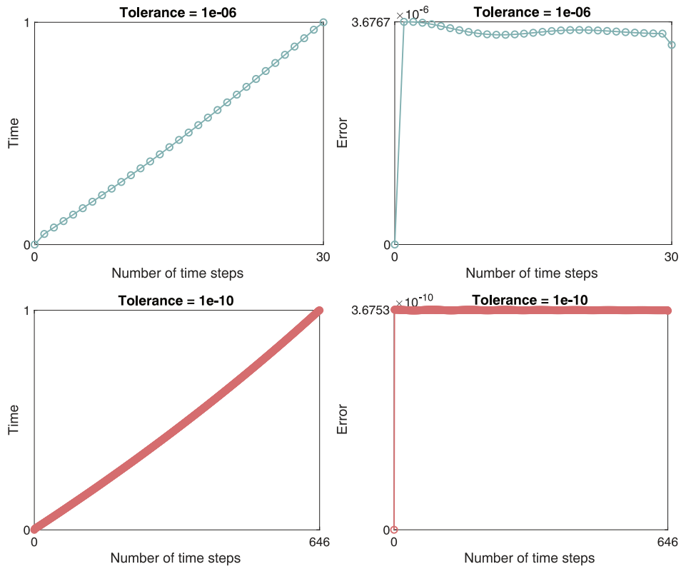
FIGURE 7. Corresponding results for the third-order symmetric-conjugate splitting method with respect to the maximum norm.
