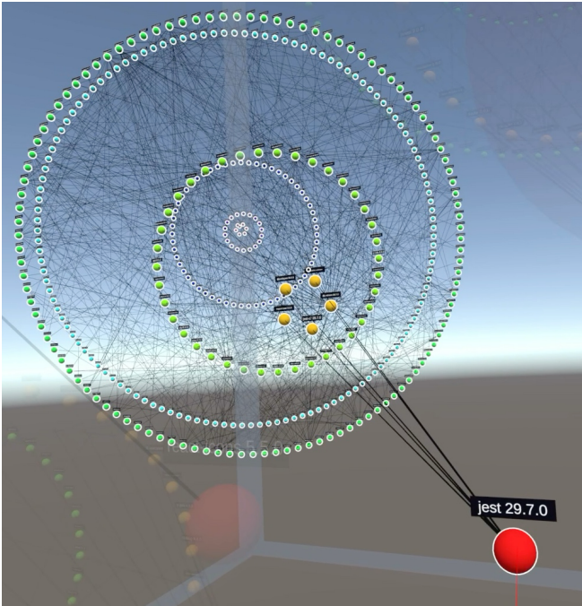
Figure 18. Git: Radial Layout: selecting node shows dependencies and toggles ghosting of rest.
