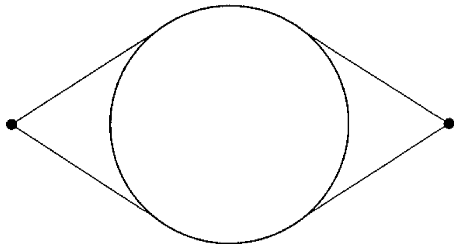
Figure 6: The new unit ball in Proposition 20
