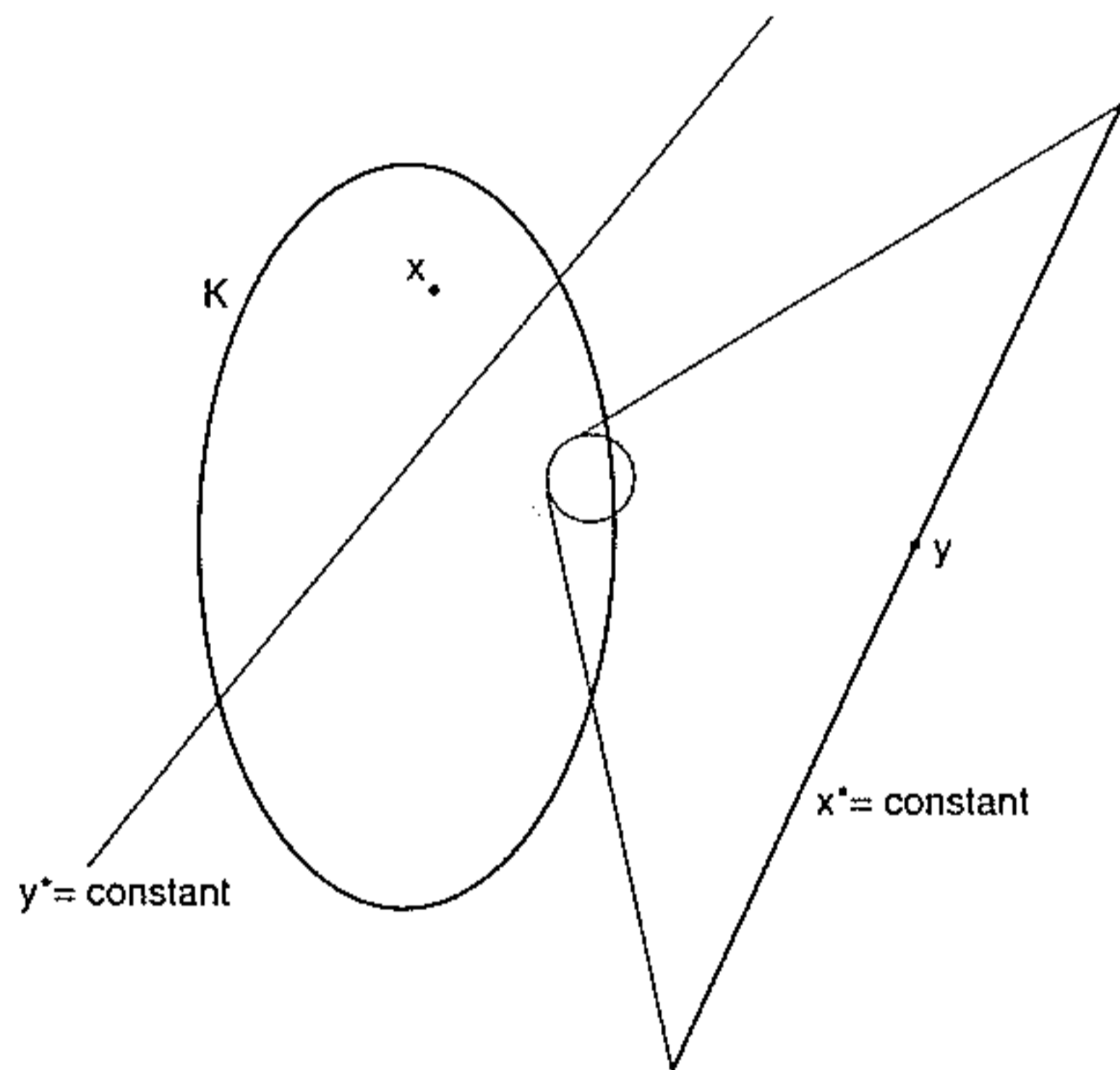
Figure 3: Prof of Theorem 7
