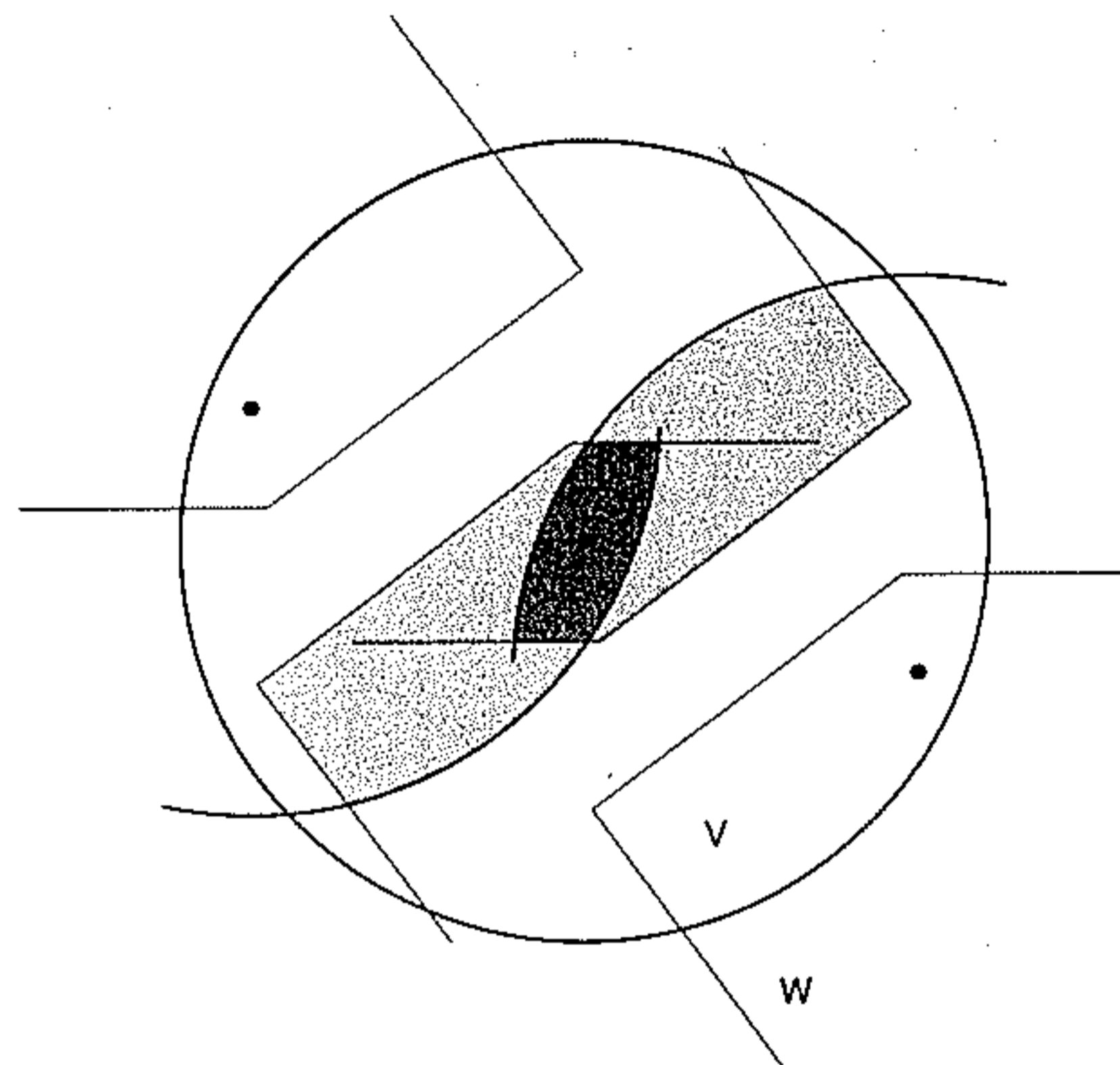
Figure 5: The new dual ball in Theorem 19
