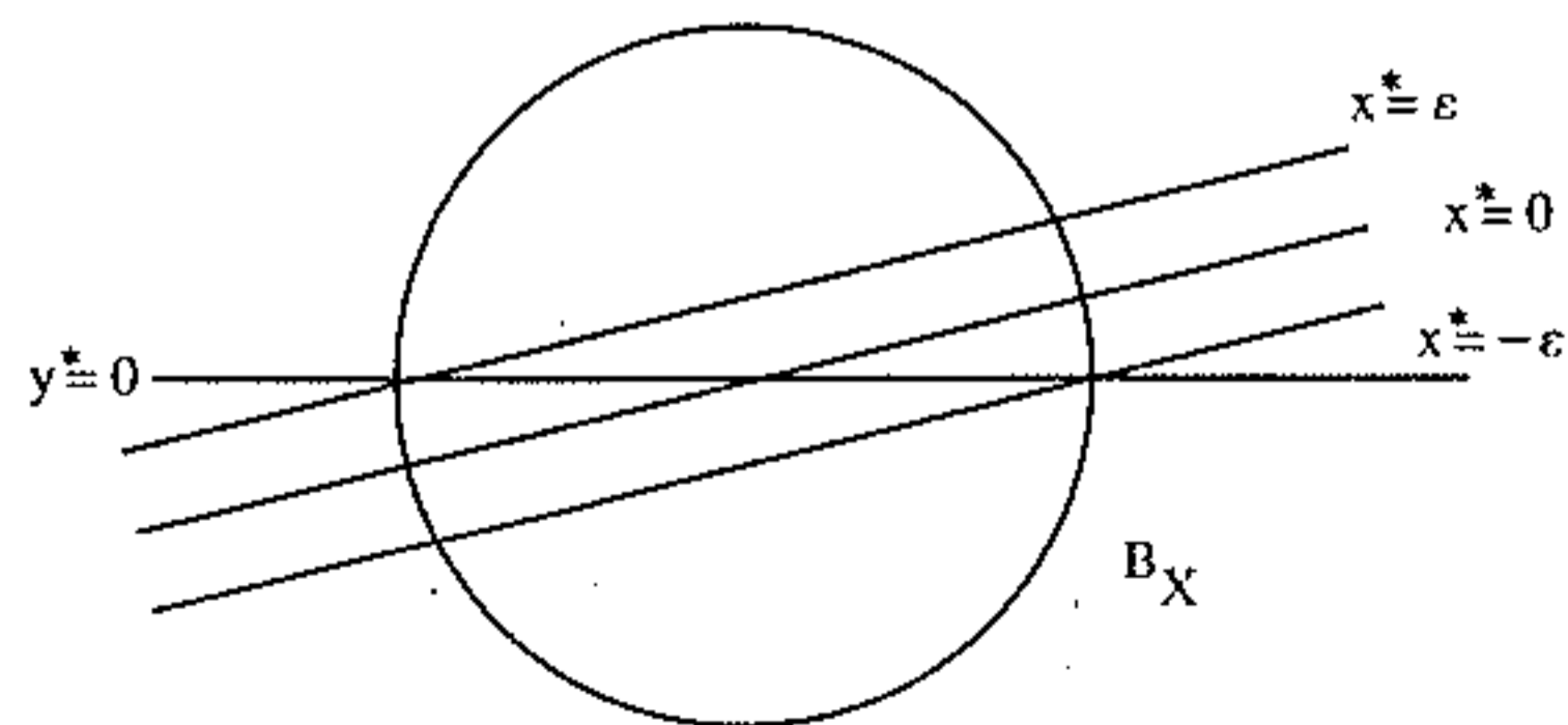
Figure 1: The Parallel Hyperplane Lemma
