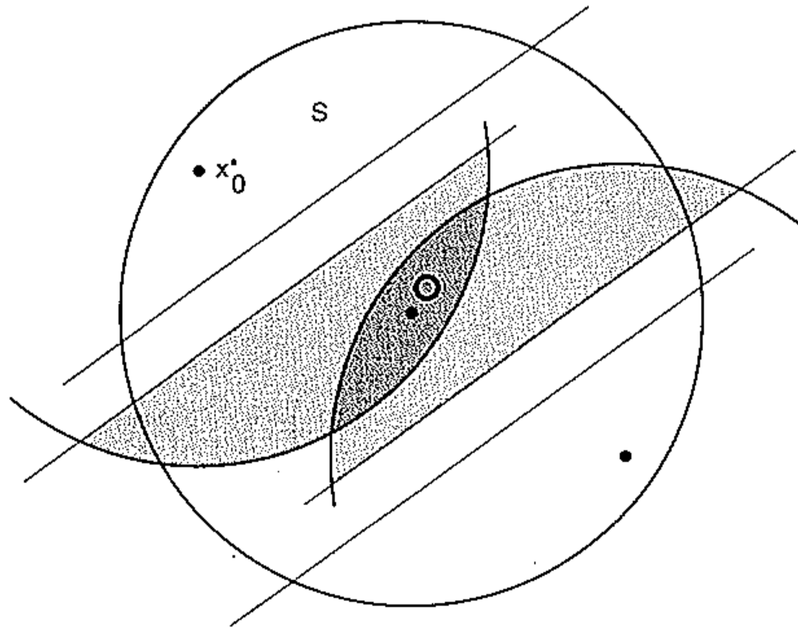
Figure 4: The new dual ball in Proposition 13
