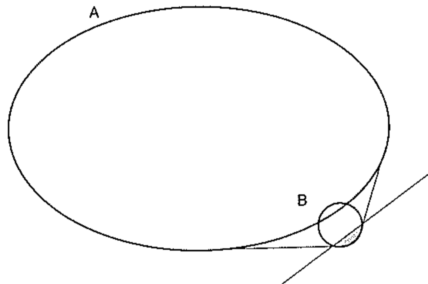
Figure 2: The Superlemma
