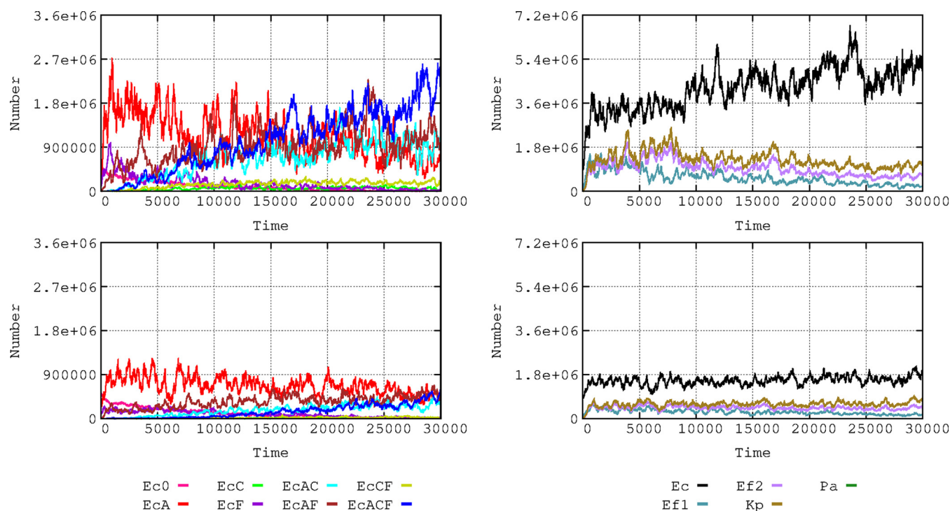
FIG 10 Influence of the intensity of the antibiotic effect on colonic microbiota of patients in the hospital. (Left) Effects on E. coli phenotype of a reduction in microbiota of 25% for AbA, 20% for AbC, and 10% for AbF (top); these values were reduced to 10%, 5%, and 2%, respectively (bottom). (Right) The effects on the species composition.
