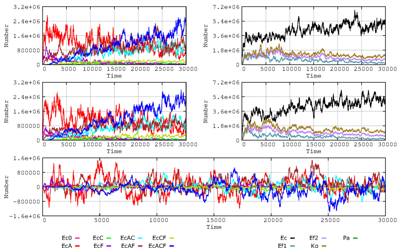
FIG 8 Influence of the frequency of bacterial cross-transmission rates in the hospital. On the left, dynamics of E. coli phenotypes when bacterial exchanges between patients occurred in 5% (top) or 20% (middle) per hour. On the right, influence on the species composition: 5% (top) or 20% (middle). A subtractive representation (5% versus 20%) is provided at the bottom. Colors are as described for Fig. 1 and 2.
